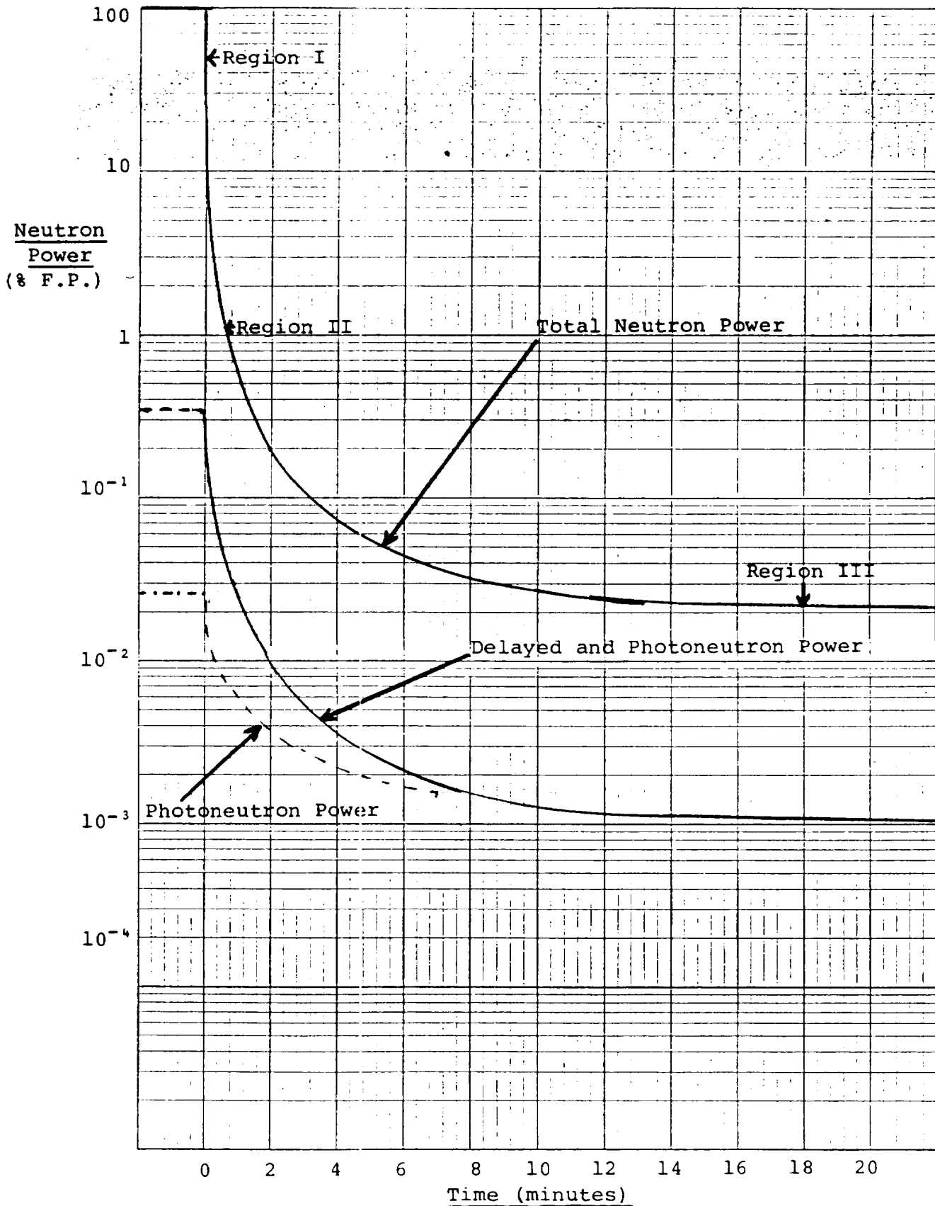
Figure 2 Neutron Power Rundown After Shutdown
