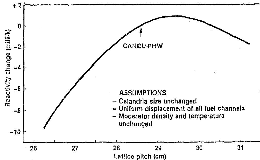
Figure 1-1: Variation of Reactivity with Lattice Pitch for CANDU-PHW Lattice.
