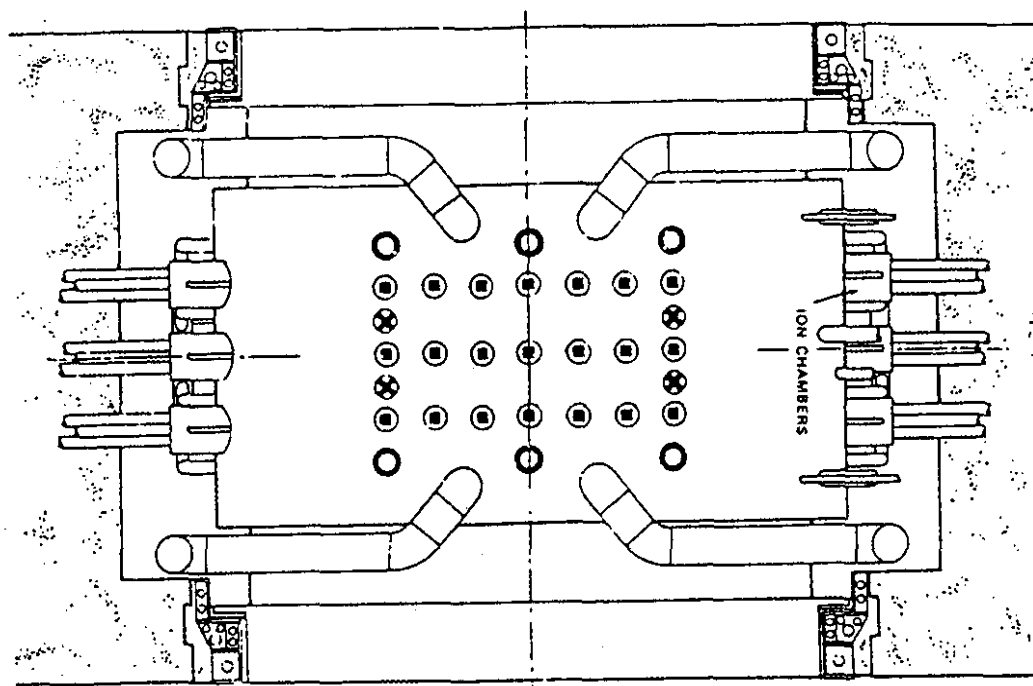
⊗ Mechanical Control Absorber Rods
