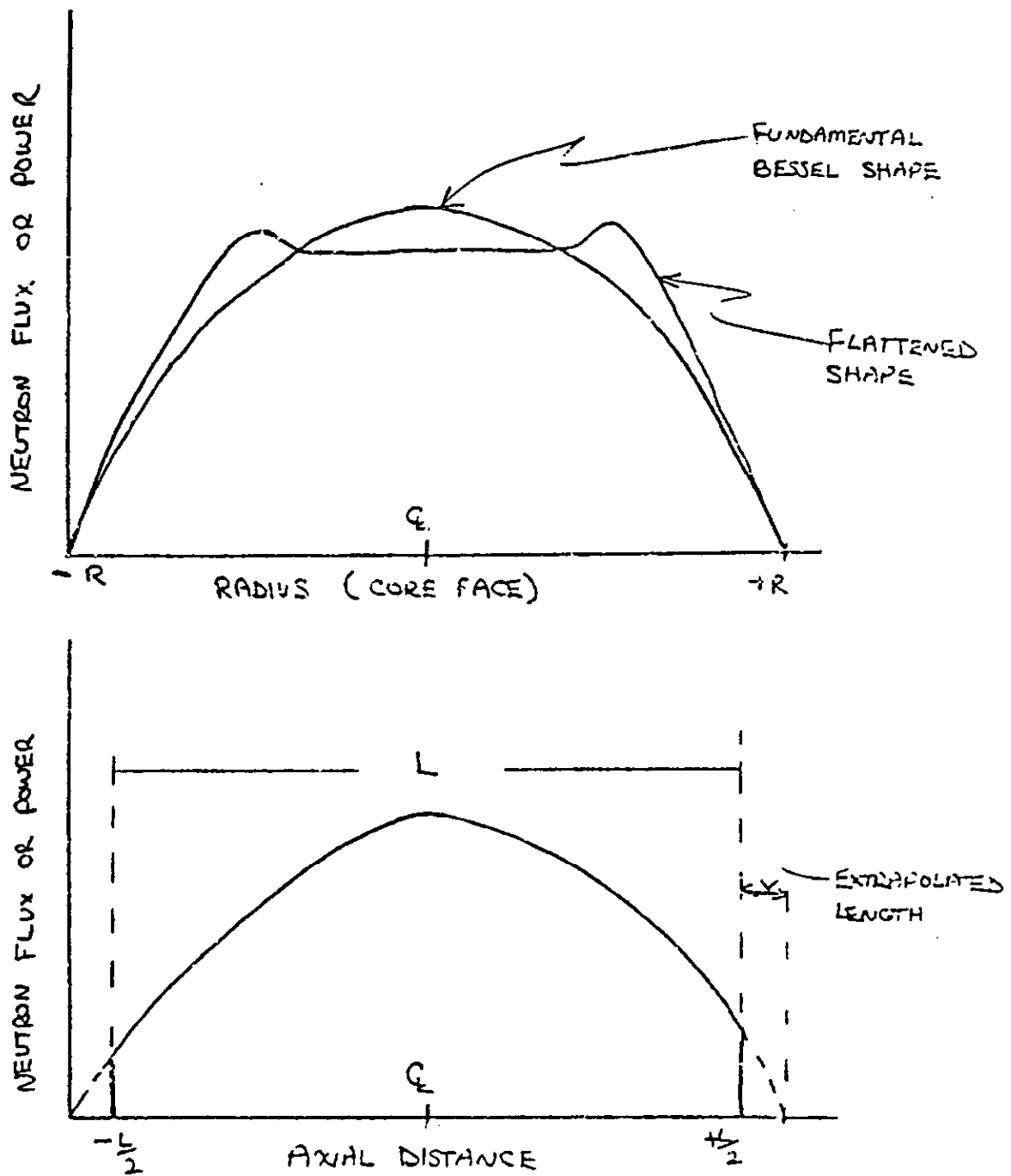
Figure 7.4 Typical power distributions.
