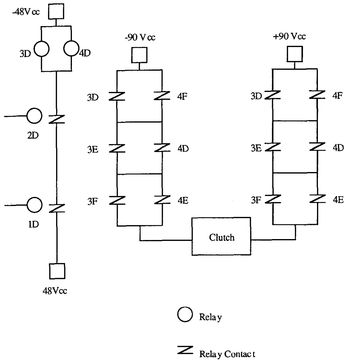
Figure 12.1: Simplified Example of two of three relay logic of SDS1
