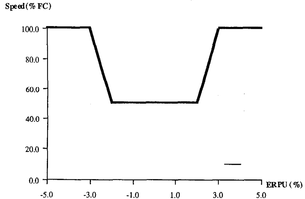
Figure 6.2: Adjuster Speed Calculation
