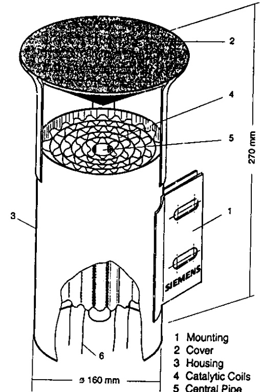
Catalytic igniter.
