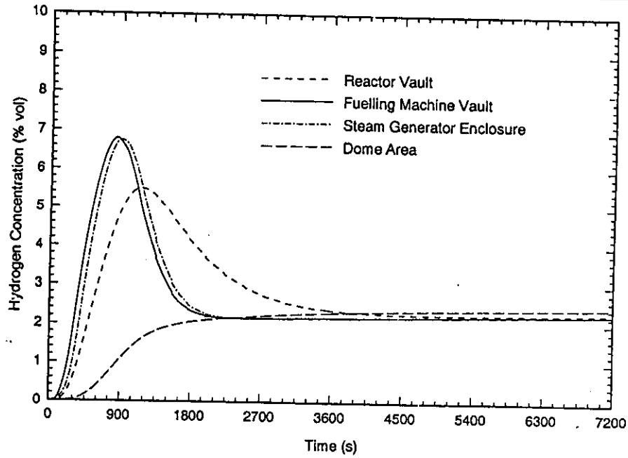
Figure 8. Preliminary estimates of hydrogen concentration in key rooms.
