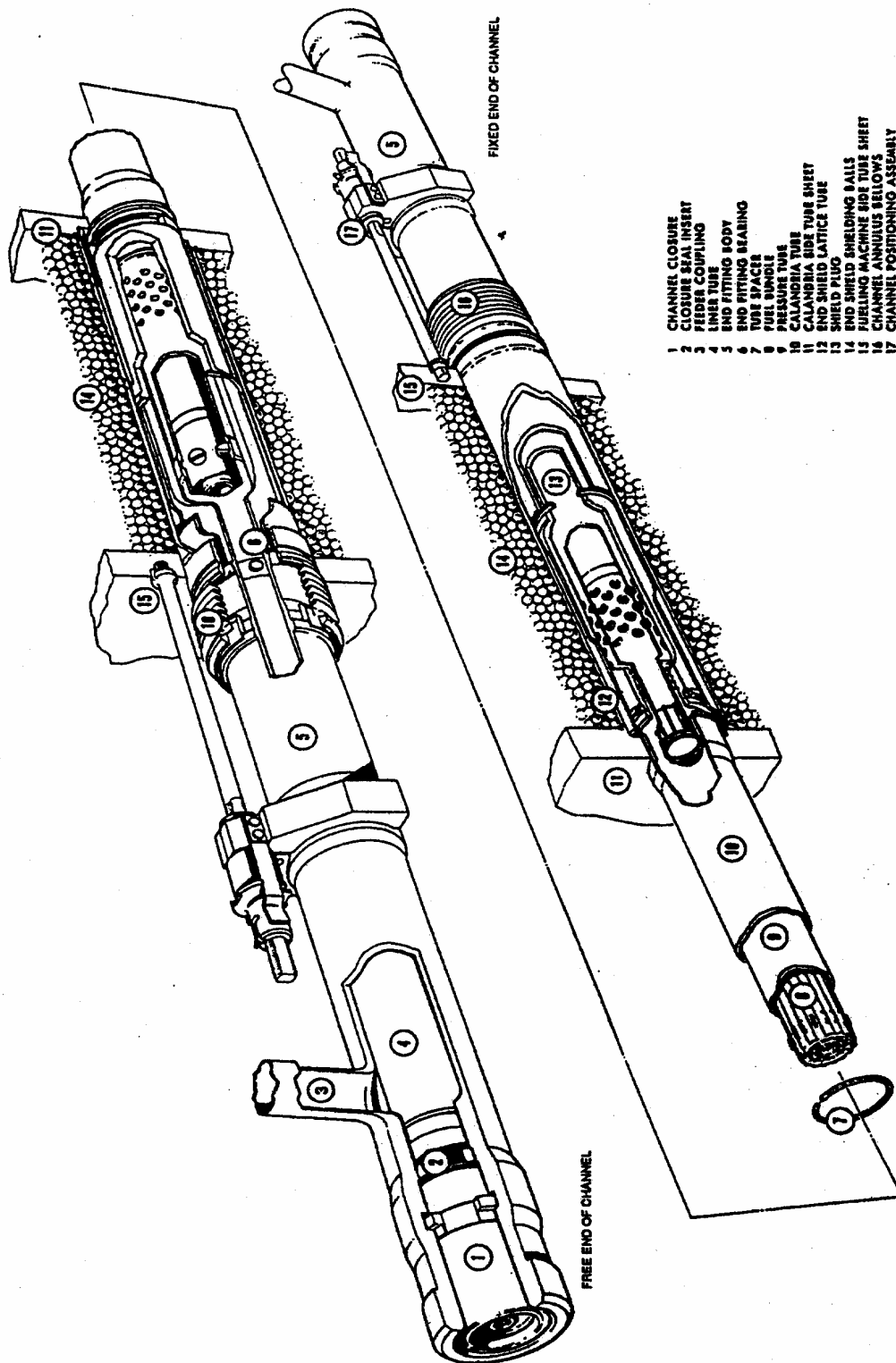
Figure 2.7. Fuel Channel Assembly.
